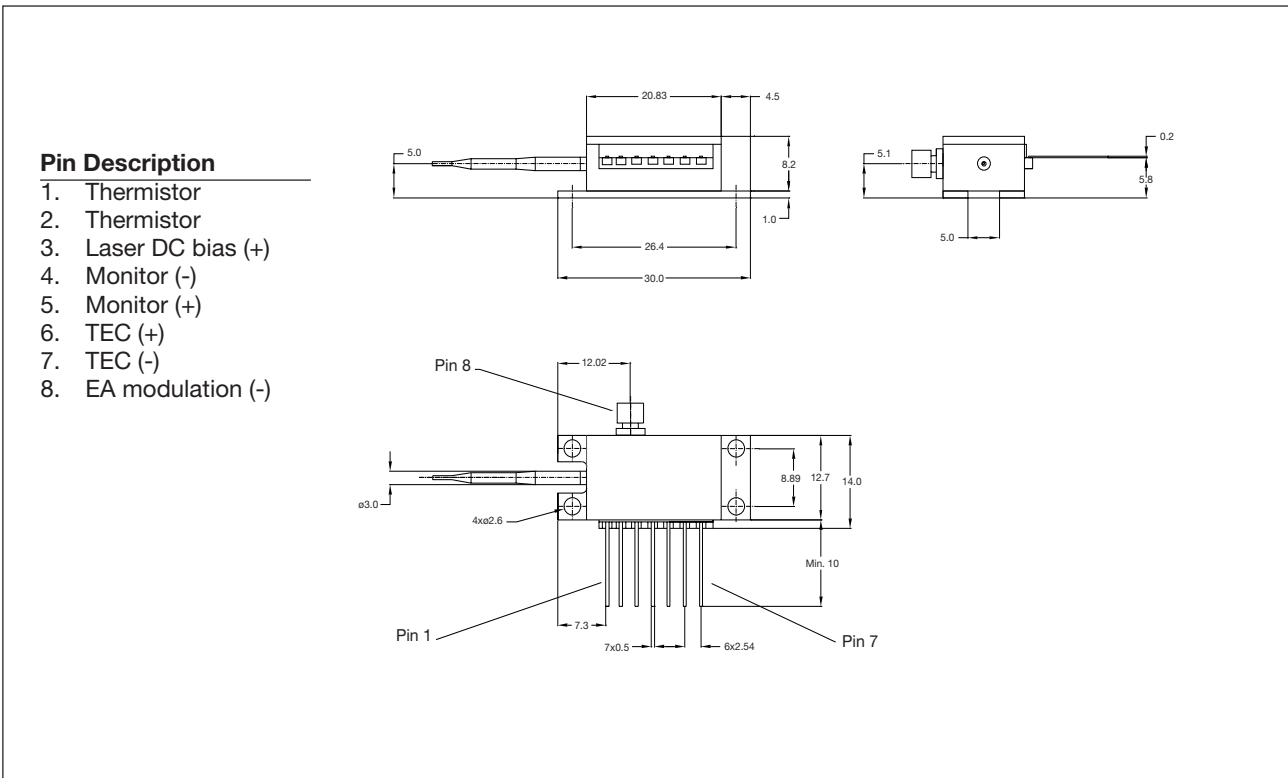
Figure 2. Pin description
