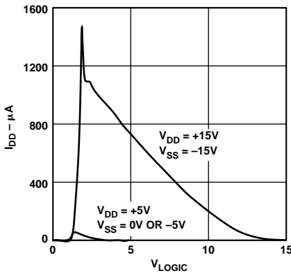
Figure 30. Supply Current ( I_{DD} ) vs. Logic Voltage
