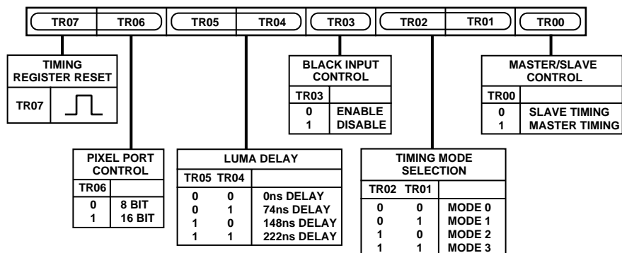
Figure 43. Timing Register 0
