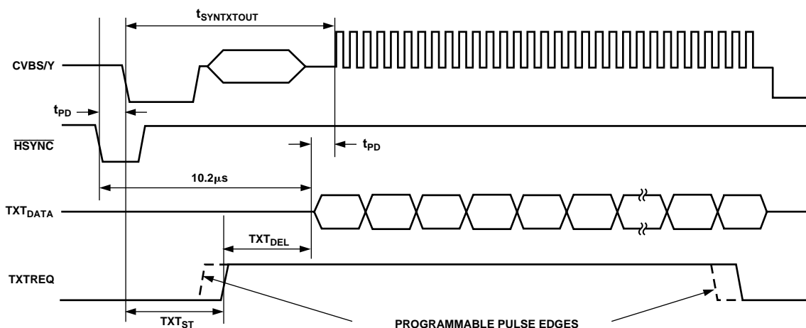
Figure 59. Teletext VBI Line
