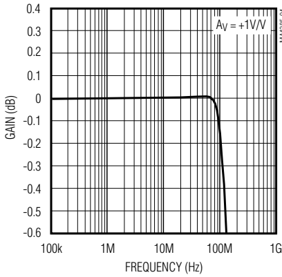
MAX4285/MAX4287/MAX4288 GAIN FLATNESS vs. FREQUENCY ( R_{LOAD} = 300\Omega )
