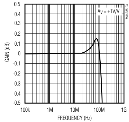
MAX4285/MAX4387/MAX4288 GAIN FLATNESS vs. FREQUENCY ( R_{LOAD} = 100\Omega )
