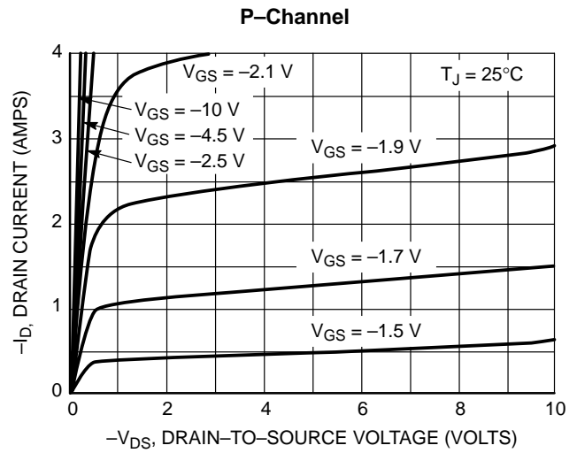
Figure 1. On-Region Characteristics
