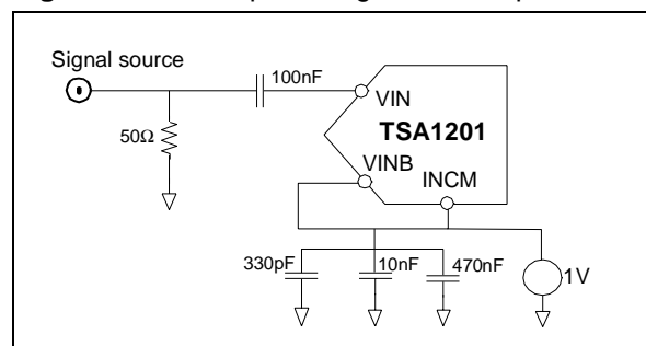
Figure 2 : AC-coupled Single-ended input
