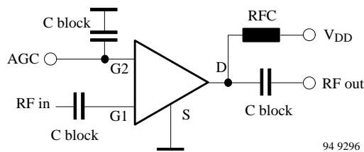
Amplifier 1
