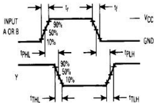
Figure 1. Switching Waveforms
