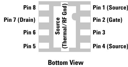
Figure 11. LPCC Package for ATF-521P8.
