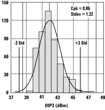
Figure 3. OIP3 @ 2 GHz, 4.5 V, 200 mA. Nominal = 41.9 dBm, LSL = 38.5 dBm.
