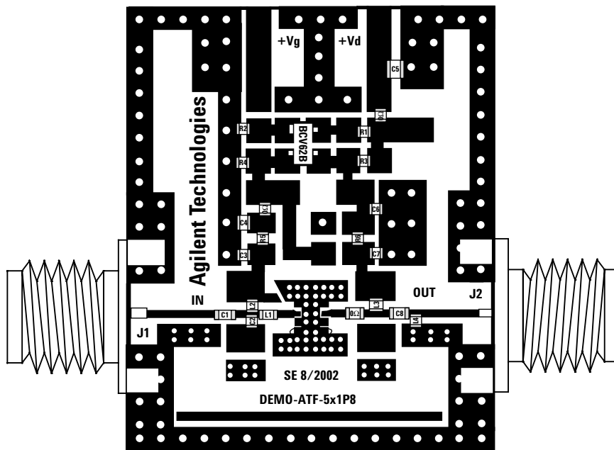
Figure 12. ATF-521P8 demoboard.
