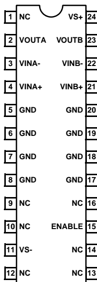
EL1506 (24-PIN SO) TOP VIEW
