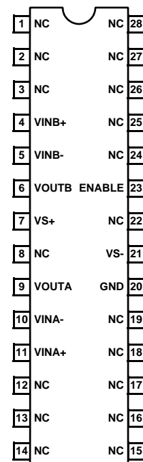
EL1506 (28-PIN HTSSOP) TOP VIEW
