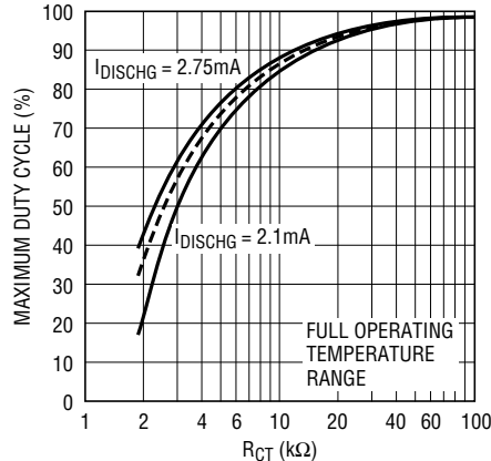
Maximum Duty Cycle vs R_{CT}
