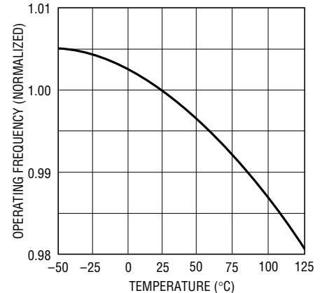
Operating Frequency (Normalized) vs Temperature
