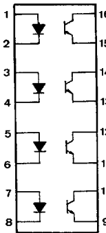
Pin No. and internal connection diagram
