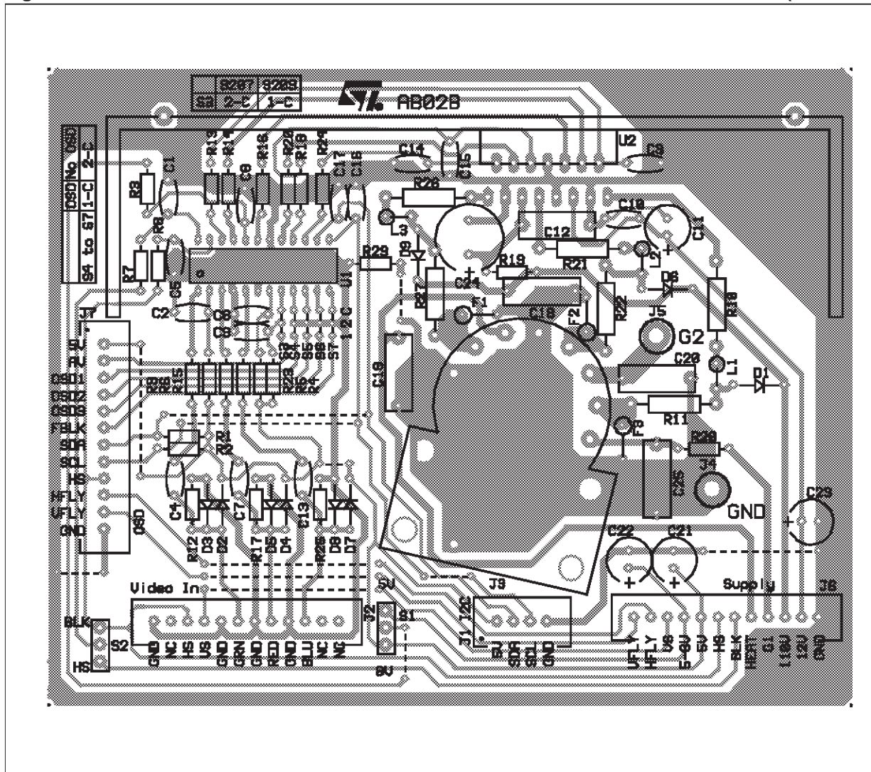
Figure 24. TDA9209/9207 - TDA9533/9530 Demonstration Board: Silk Screen and Trace (scale 1:1)
