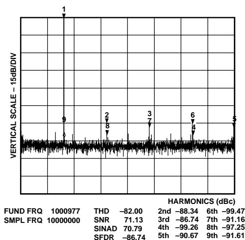
Figure 40. FFT of AD9220 Output When Driven by AD8042
