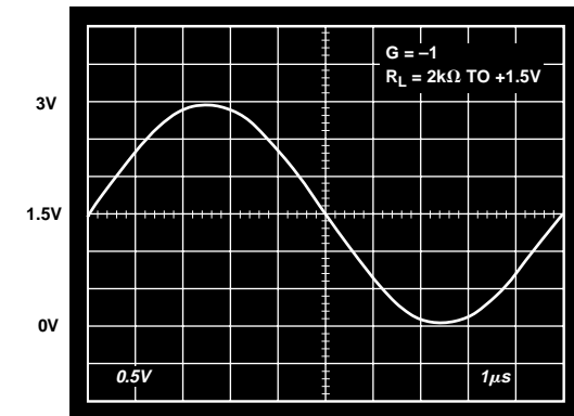
Figure 31. Rail-to-Rail Output Swing, V_S = +3 V
