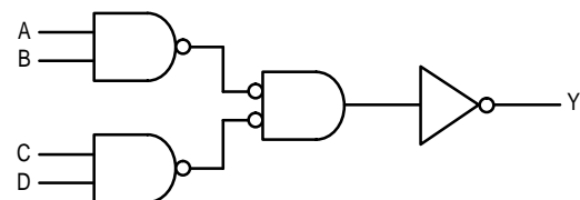
EXPANDED LOGIC DIAGRAM (1/2 OF THE DEVICE)
