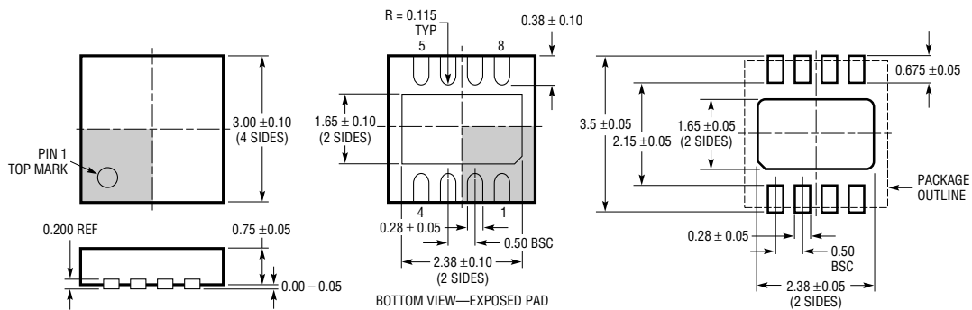
RECOMMENDED SOLDER PAD PITCH AND DIMENSIONS (028) DFN 0203
