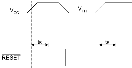
Figure 1: Timing Diagram
