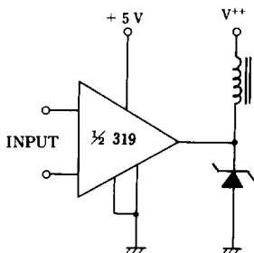
Relay Driver
