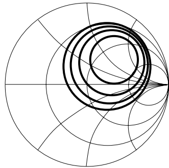
Figure 19. Noise Circles F = 1900 \text{ MHz} , Step Size: 0.2 \text{ dB} .
