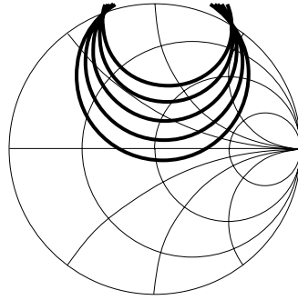
Figure 20. Gain Circle F = 1900 \text{ MHz} , Step Size: 1.0 \text{ dB} .
