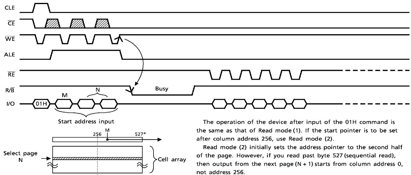
Figure 4. Read mode (2) operation
