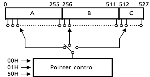
Figure 8. Pointer control
