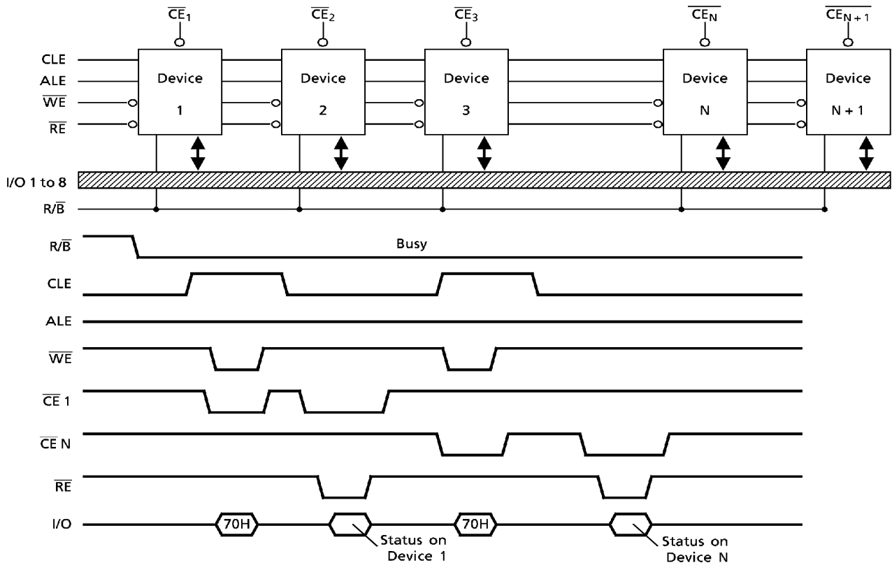
Figure 6. Status read timing application example
