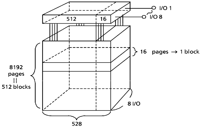
Figure 2. Schematic Cell Layout
