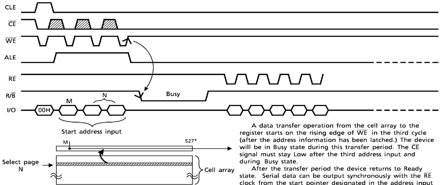
Figure 3. Read mode (1) operation
