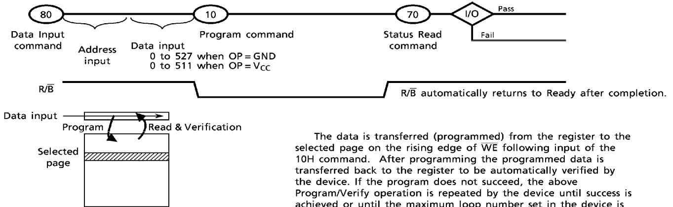
Figure 7. Auto Page Program operation
