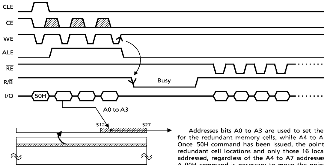
Figure 5. Read mode (3) operation
