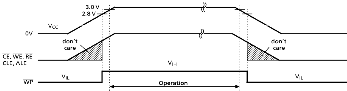
Figure 10. Power On/Off Sequence
