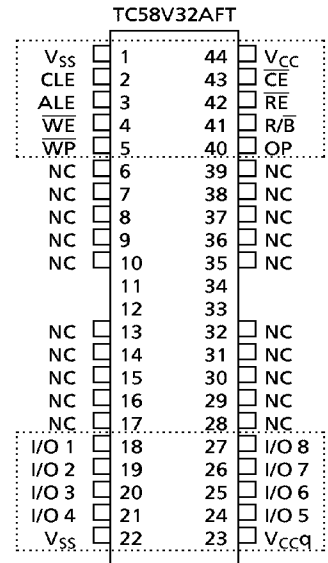
Figure 1. Pinout
