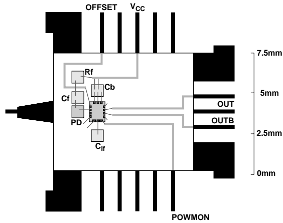
Figure 19. Butterfly Package
