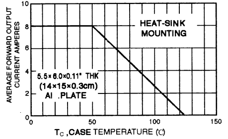
FIG. 2 - TYPICAL FORWARD OUTPUT CURRENT DERATING CURVE
