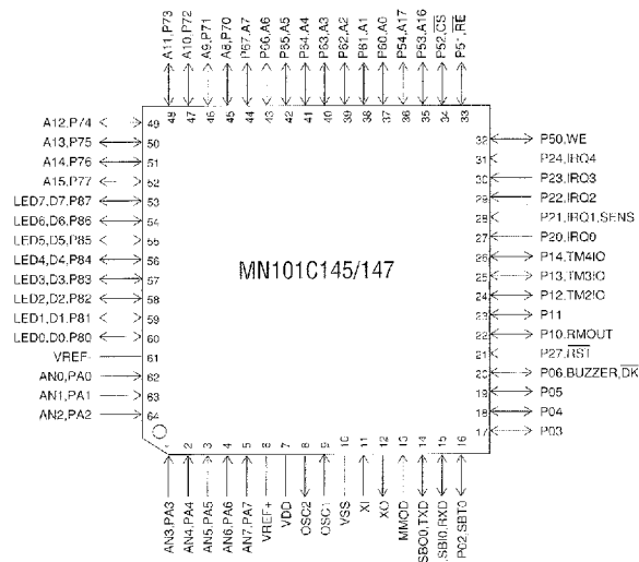
LQFP064-P-1414
