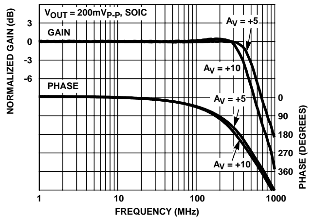
FIGURE 13. FREQUENCY RESPONSE
