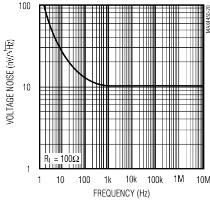
MAX4450 VOLTAGE NOISE vs. FREQUENCY
