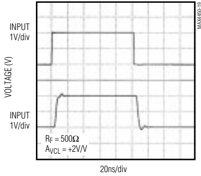
MAX4450 LARGE-SIGNAL PULSE RESPONSE
