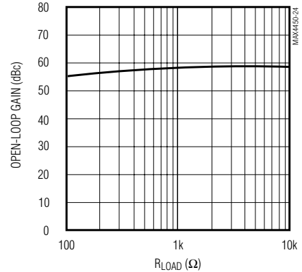
MAX4450 OPEN-LOOP GAIN vs. RESISTIVE LOAD
