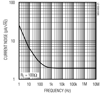
MAX4450 CURRENT NOISE vs. FREQUENCY
