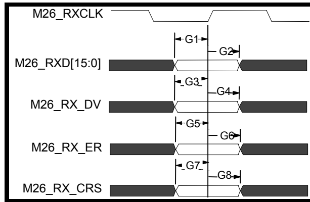
Figure 29 - AC Characteristics – Gigabit Media Independent Interface
