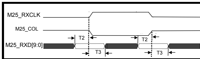
Figure 27 - Gigabit TBI Interface Receive Timing
