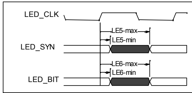
Figure 32 - AC Characteristics – LED Interface
