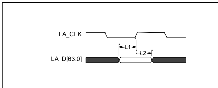
Figure 18 - Local Memory Interface – Input setup and hold timing
