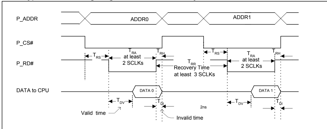
Figure 17 - Typical CPU Timing Diagram for a CPU Read Cycle
