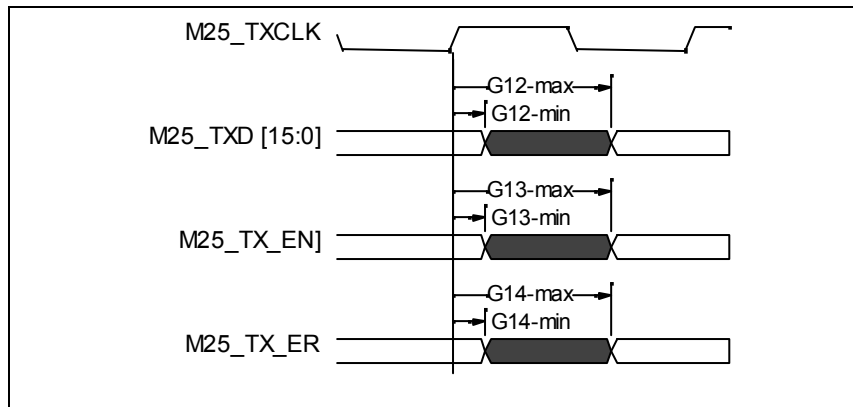
Figure 24 - AC Characteristics- GMII
