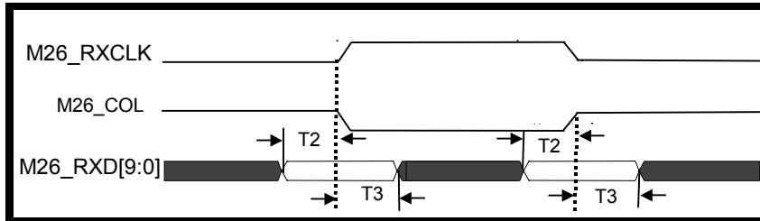
Figure 31 - Gigabit TBI Interface Timing
