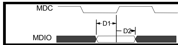
Figure 35 - MDIO Input Setup and Hold Timing
