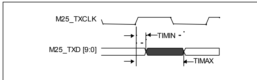
Figure 26 - Gigabit TBI Interface Transmit Timing
