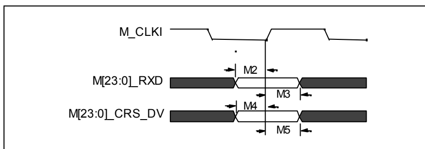
Figure 23 - AC Characteristics – Reduced Media Independent Interface
