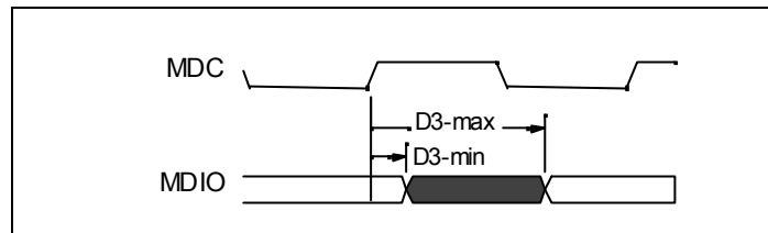
Figure 36 - MDIO Output Delay Timing
