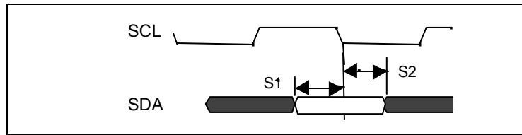
Figure 37 - I 2 C Input Setup Timing
