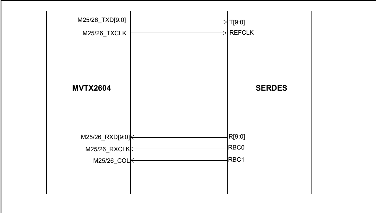
Figure 12 - TBI Connection
