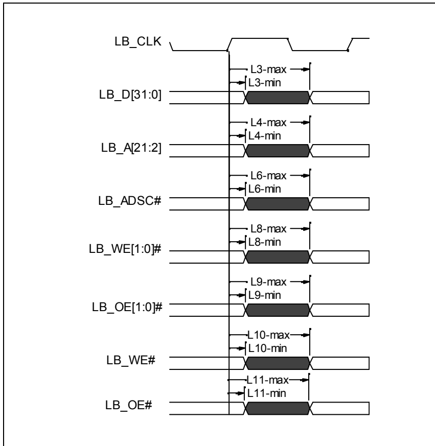
Figure 21 - Local Memory Interface - Output valid delay timing
