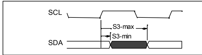
Figure 38 - I 2 C Output Delay Timing
