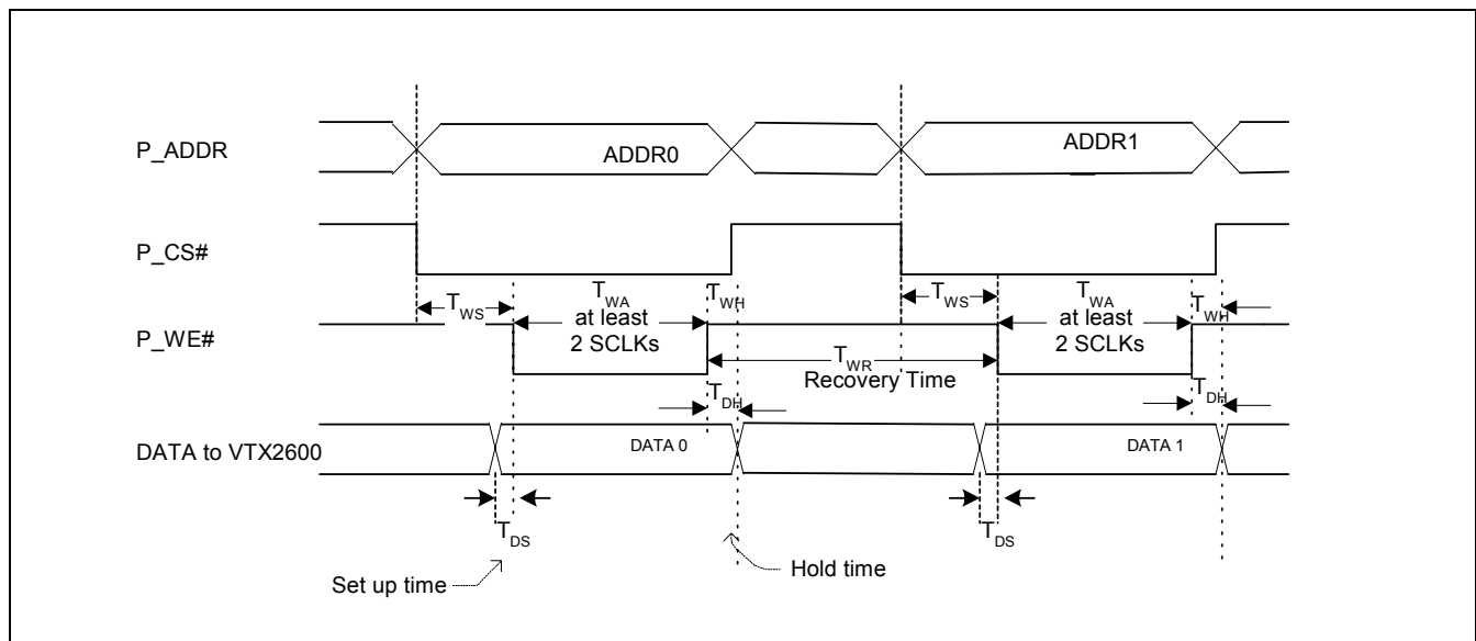
Figure 16 - Typical CPU Timing Diagram for a CPU Write Cycle
