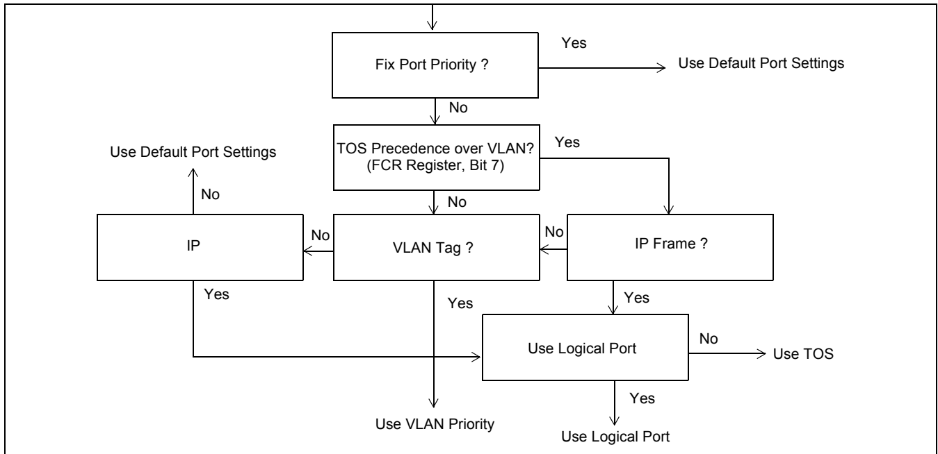
Figure 5 - Priority Classification Rule
