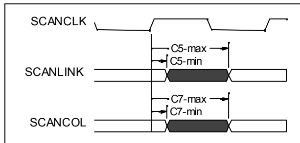
Figure 33 - SCANLINK SCANCOL Output Delay Timing
