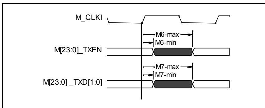
Figure 22 - AC Characteristics – Reduced media independent Interface
