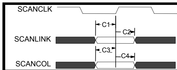
Figure 34 - SCANLINK, SCANCOL Setup Timing
