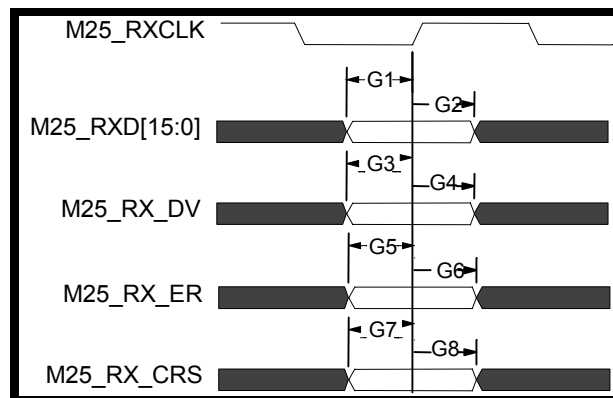
Figure 25 - AC Characteristics – Gigabit Media Independent Interface
