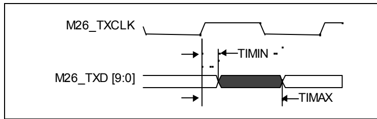
Figure 30 - Gigabit TBI Interface Transmit Timing
