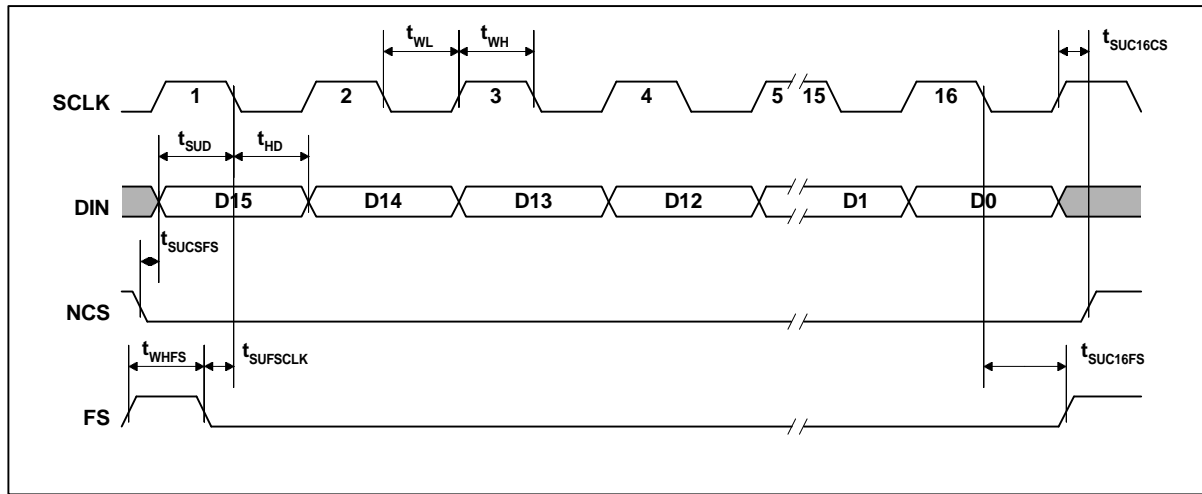
Figure 1 Timing Diagram
