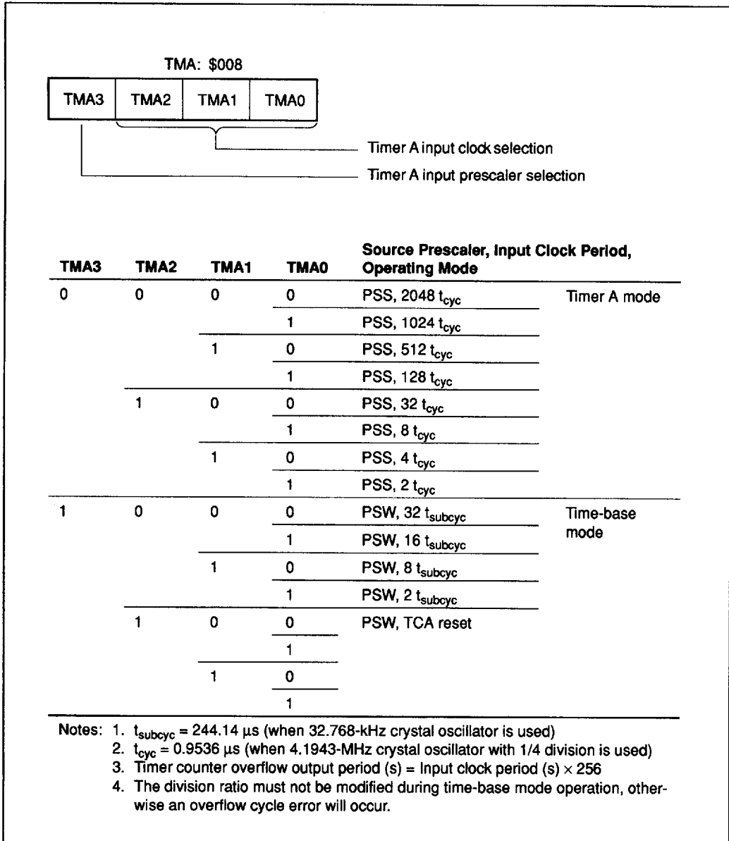
Figure 29 Timer Mode Register A
