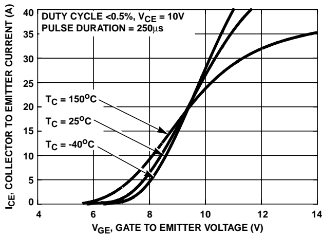
FIGURE 1. TRANSFER CHARACTERISTICS
