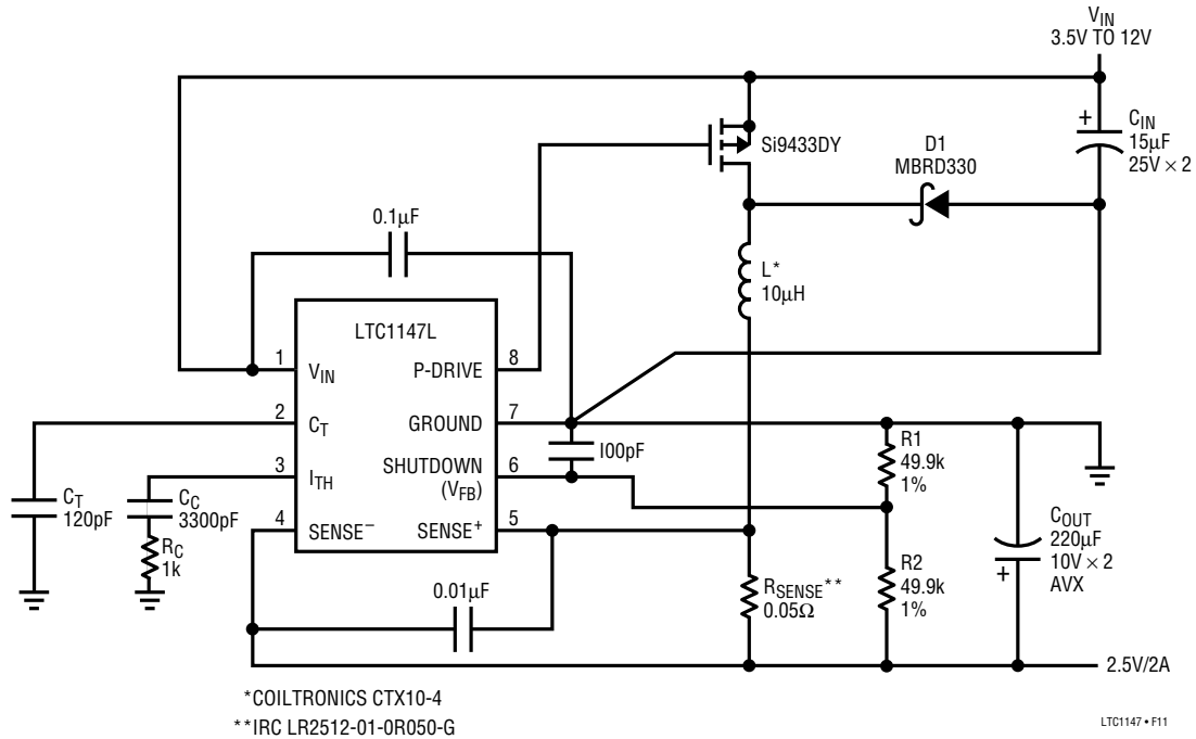
Figure 11. 2.5V, 2A Regulator
