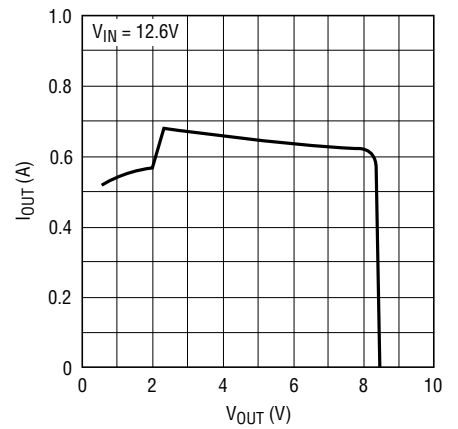
Figure 10. I OUT vs. V OUT For Figure 9.
