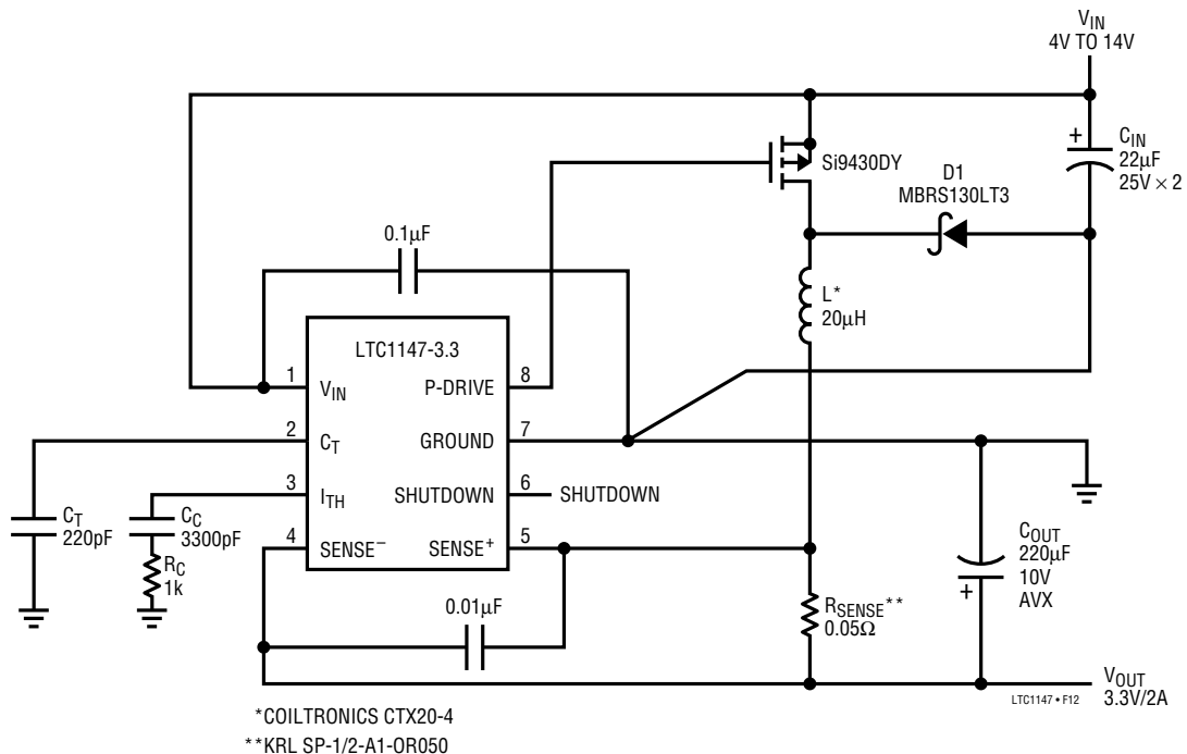
Figure 12. 3.3V, 2A Output High Efficiency Regulator
