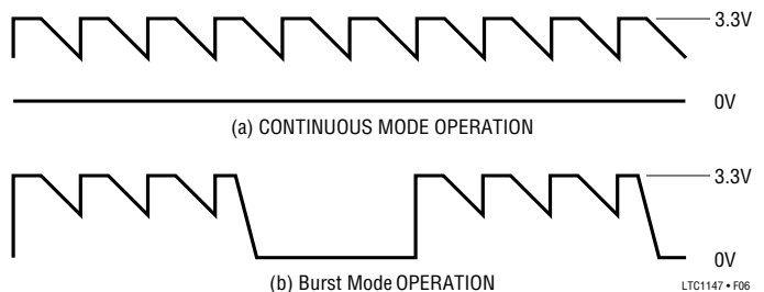
Figure 6. C_T Waveforms
