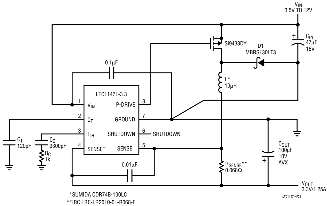
Figure 8. 3.3V Low Dropout High Efficiency Regulator
