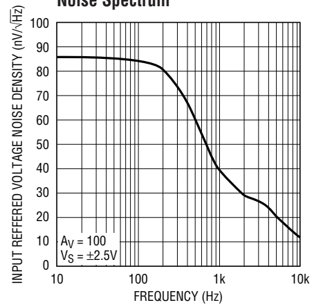
Noise Spectrum
