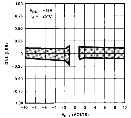
DIFFERENTIAL NONLINEARITY vs V_{REF}
