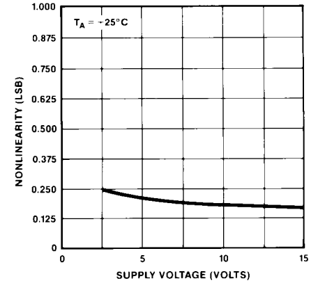
NONLINEARITY vs V_{DD}
