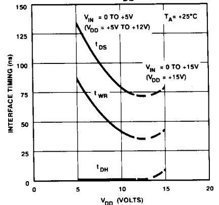
INTERFACE TIMING vs V DD
