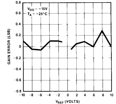
ABSOLUTE GAIN ERROR CHANGE vs V_{REF}
