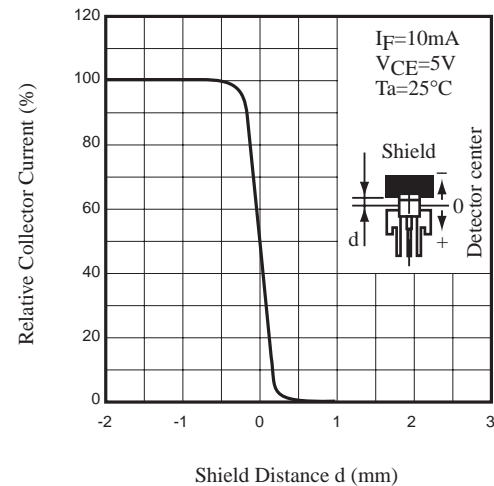
Relative Collector Current vs. Shield Distance (2)
