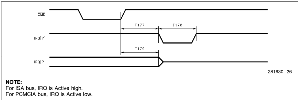
Figure 11-16. Interrupt Timing
