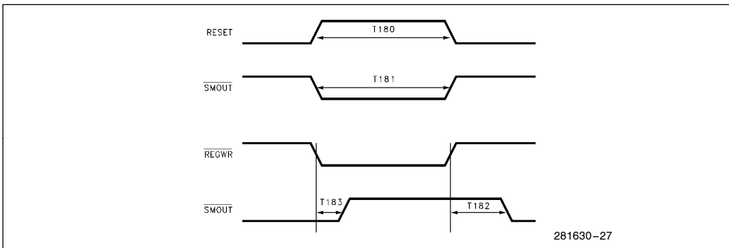
Figure 11-17. \overline{SMOUT} Timing
