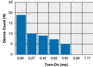
IAB110P - FormB Typical Turn-On Time (N=50 Ambient Temperature = 25°C) (Load Current = 100mADC; I F = 5mADC)
