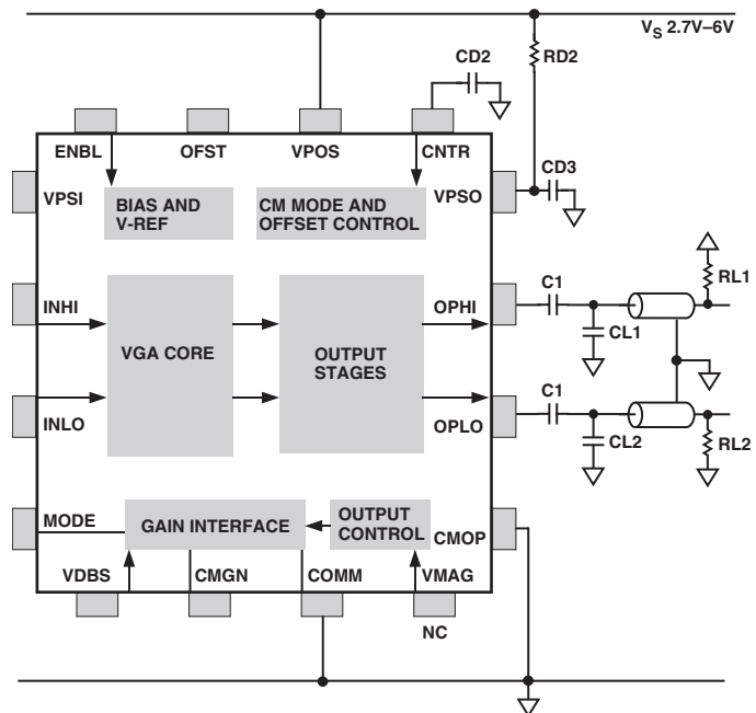
Figure 18. Driving Dual Cables with Grounded Loads
