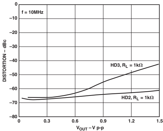
TPC 22. Harmonic Distortion vs. V_{OUT-DIFFERENTIAL} V_{MAG} = 0.5 V
