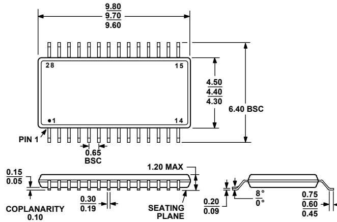
Figure 48. 28-Lead Thin Shrink Small Outline Package [TSSOP] (RU-28) Dimensions shown in millimeters
