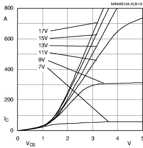
Fig. 10 Typ. output characteristic, t_p = 80 \mu s ; 125 \text{ }^\circ\text{C}
