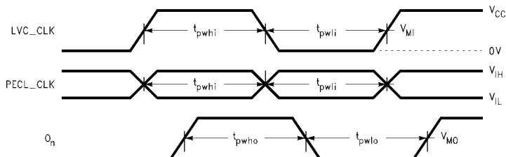
FIGURE 4. Duty Cycle Distortion dpwh = (t_{pwho} - t_{pwhi}) ; dpwl = (t_{pwl0} - t_{pwl1})
