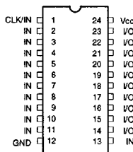
DIP/SOIC
