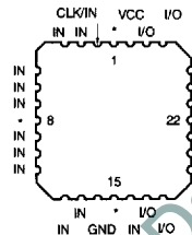
PLCC
