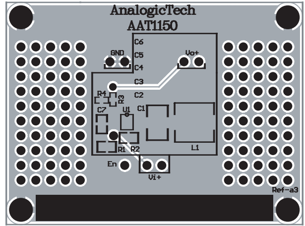
Figure 5: AAT1150 Evaluation Board Layout Bottom Layer.
