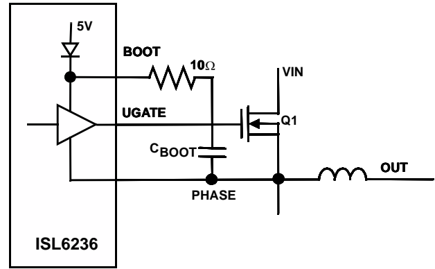
FIGURE 75. REDUCING THE SWITCHING-NODE RISE TIME
