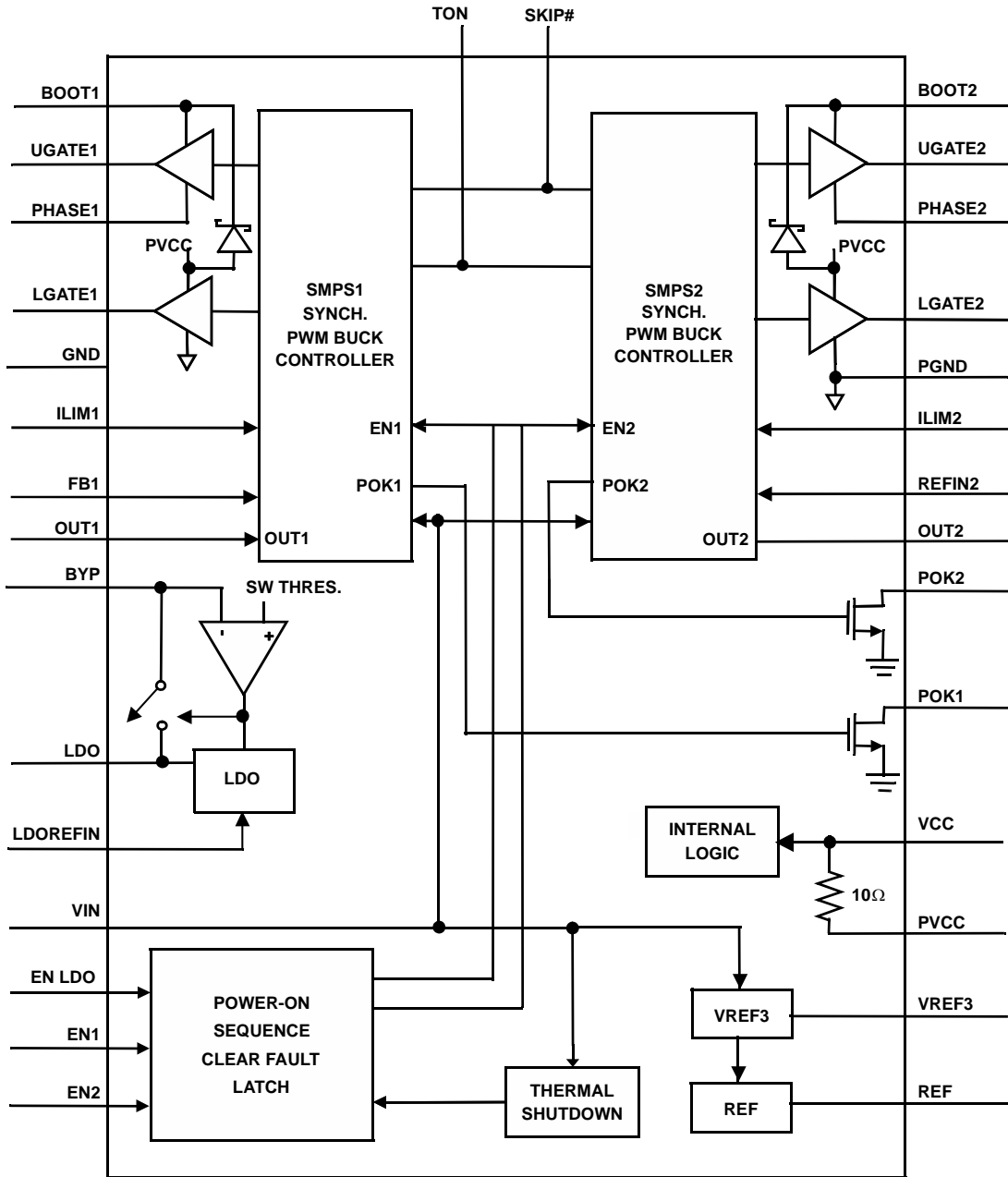
FIGURE 69. DETAIL FUNCTIONAL DIAGRAM ISL6236
