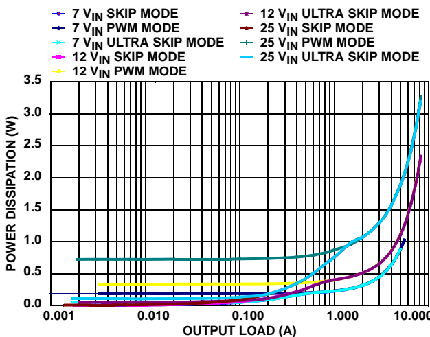
FIGURE 12. V_{OUT1} = 5V POWER DISSIPATION vs LOAD (400kHz)
