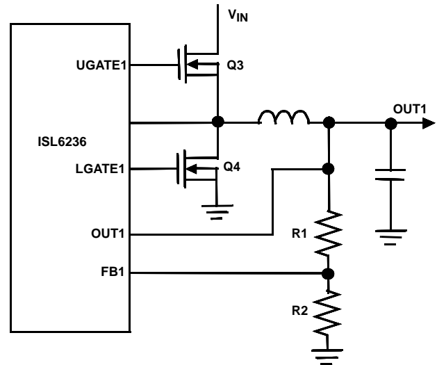
FIGURE 76. SETTING V_{OUT1} WITH A RESISTOR DIVIDER
