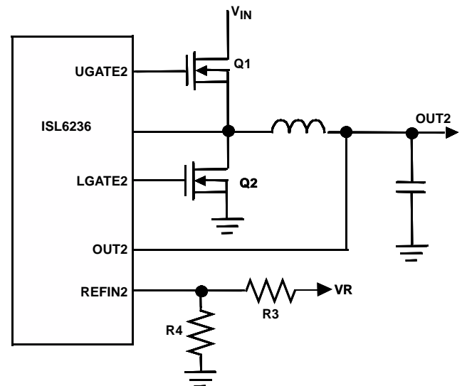
FIGURE 77. SETTING V_{OUT2} WITH A VOLTAGE DIVIDER FOR TRACKING
