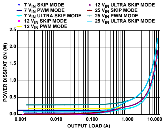
FIGURE 10. V_{OUT1} = 1.5V POWER DISSIPATION vs LOAD (200kHz)
