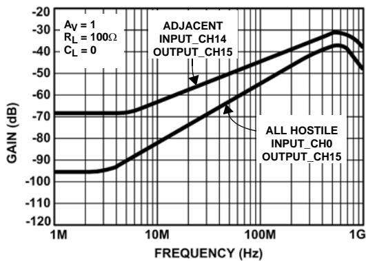
FIGURE 11. CROSSTALK - A_V = 1
