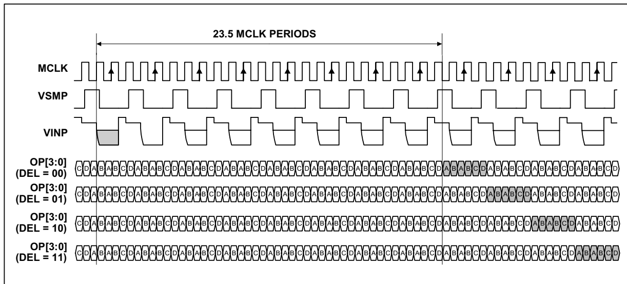
Figure 16 Mode 2 Operation
