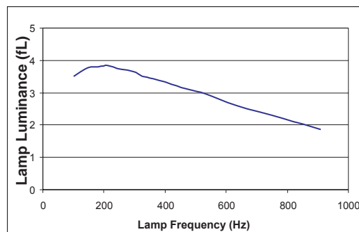
Figure 2: Typical Lamp Luminance vs. Lamp Frequency ( V^+ = 3.0V , 2.4 \text{ in}^2 Durel 3 Green EL Lamp Load)
