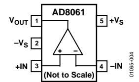
Figure 4. 5-Lead SOT-23 (RT)
