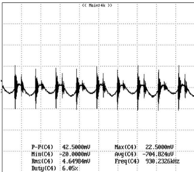
Figure 12: Input reflected ripple current, i_s , through a 12\mu\text{H} source inductor at nominal input voltage and rated load current ( 20\text{ mA/div} , 2\text{ us/div} ).
