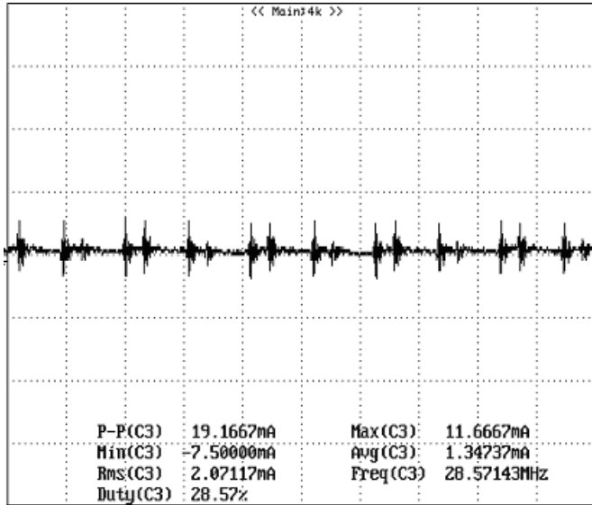
Figure 12: Input reflected ripple current, i_s , through a 12\mu\text{H} source inductor at nominal input voltage and rated load current ( 20\text{ mA/div} , 2\text{ us/div} ).
