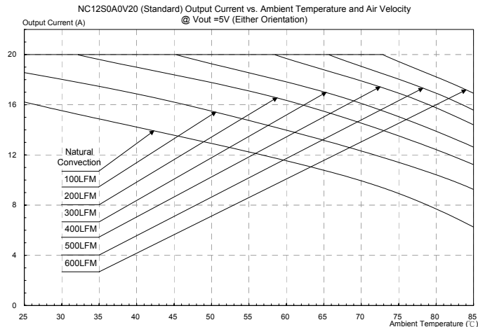
Figure 34: Output current vs. ambient temperature and air velocity @ Vout=5V (Either Orientation)
