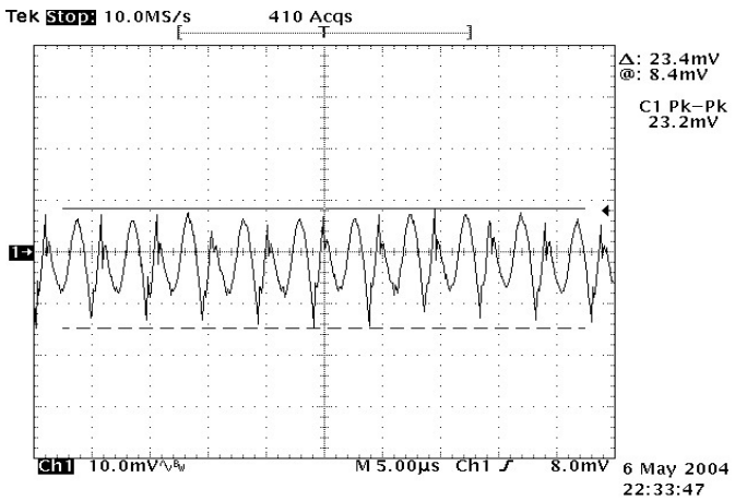
Figure 9: Output ripple & noise at 12Vin, 1.8V/20A out
