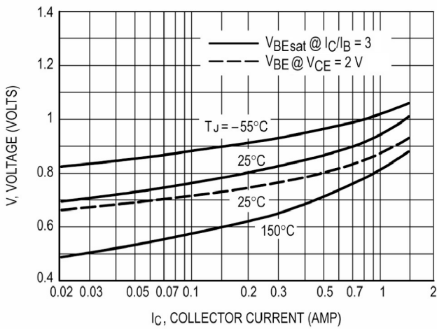
Base-Emitter Voltage
