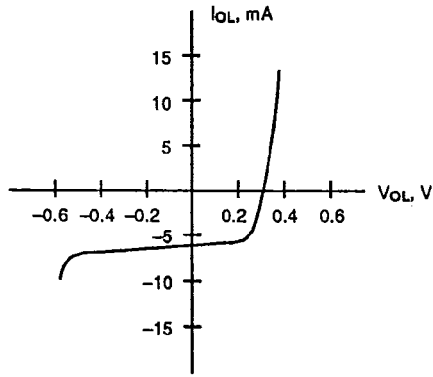
Output, LOW
