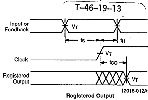
Registered Output
