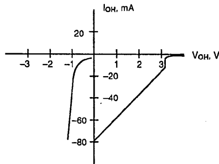
Output, HIGH
