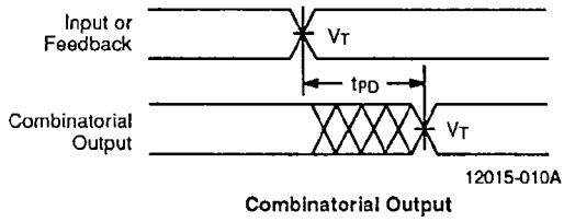
Combinatorial Output
