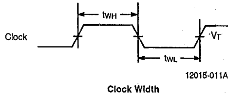
Clock Width
